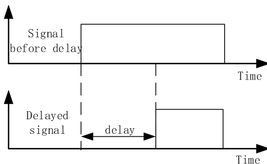
Figure 6-3-7 Y output delay
