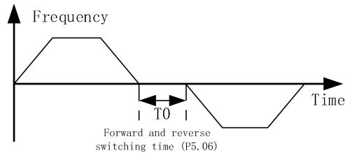
Figure 6-5-2 Switching between forward and reverse
