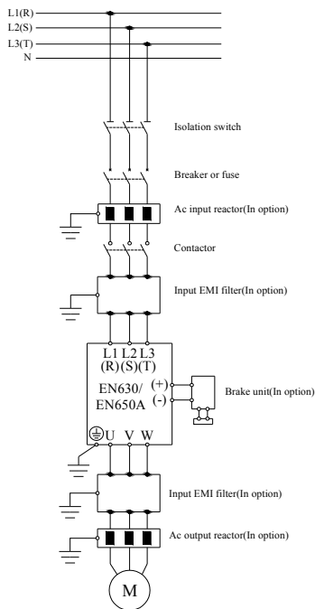
Fig.3-5 Connection of inverter and fitting parts
