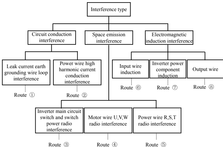
Fig.3-13 Interference noise type
