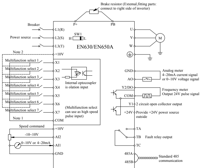
Fig.3-6 Basic wiring diagram
