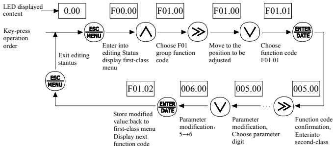
Fig.4-8 Example for parameter setting and modification
