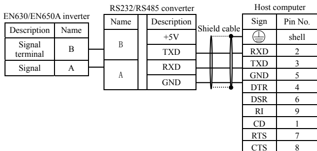
Fig.3-12 RS485 communication wiring
