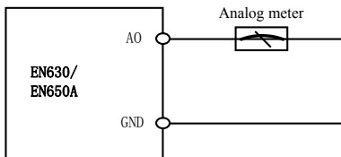
Fig.3-10 AO Terminal wiring diagram
