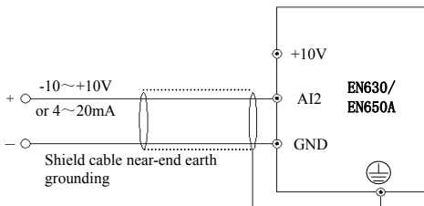
Fig.3-9 AI2 Terminal wiring diagram
