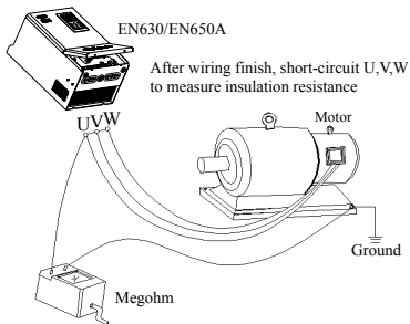
Fig.1-1 Motor insulation check
