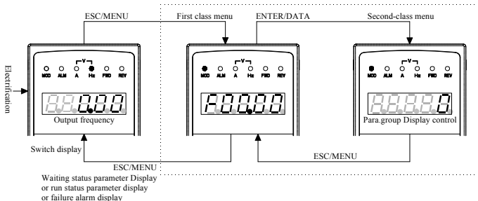
Fig.4-5 Keypad display status switching
