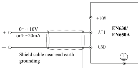
Fig.3-8 AI1 Terminal wiring diagram
