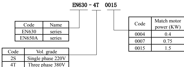
Fig.2-1 Type description
