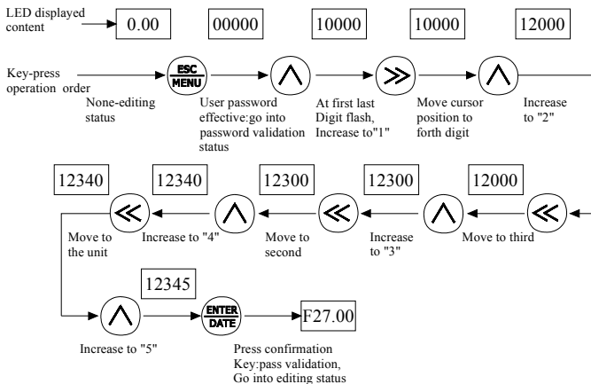
Fig.4-11 Inputting password to go into function code operation
