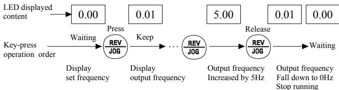
Fig.4-10 Jog run operating example
