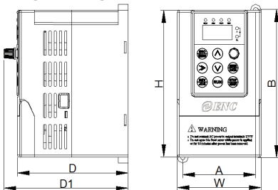
Fig.2-4 Outer dimension
