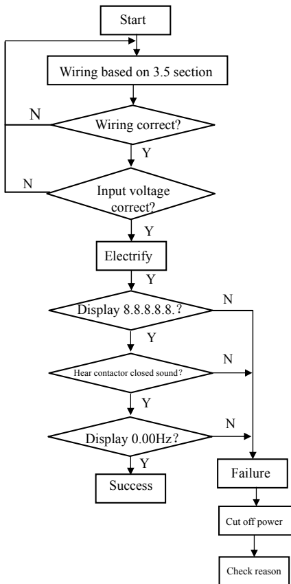
Fig.4-12 First electrification operation flow
