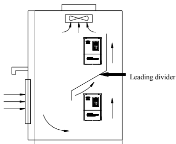
Fig.3-2 Mounting of multiple inverters
