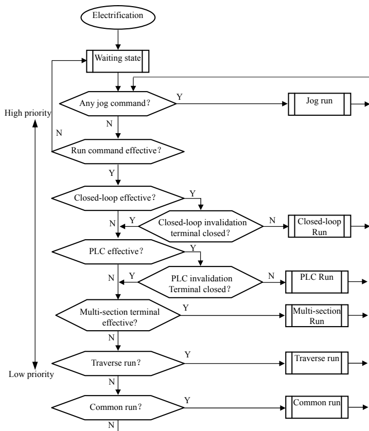
Fig.4-1 Logic flow chart of EN630/EN650A inverter running state
