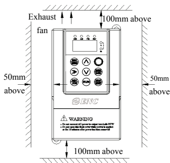
Fig.3-1 Mounting space
