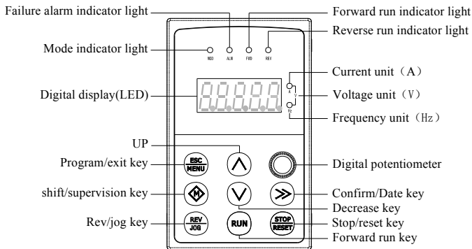
Fig.4-2 Keypad layout sketch
