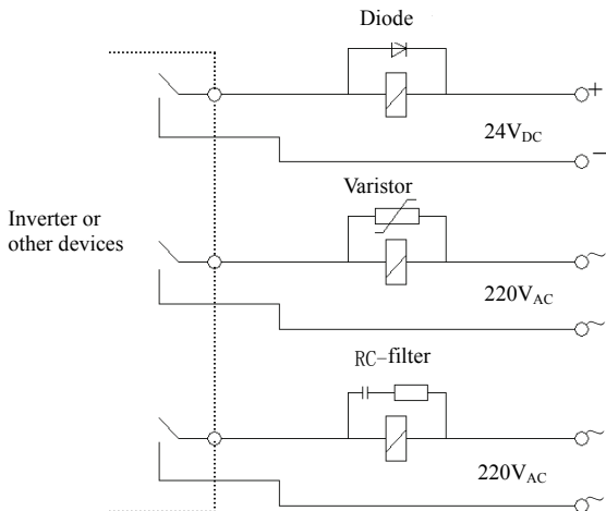
Fig.3-16 Install demand for electromagnetic on-off device
