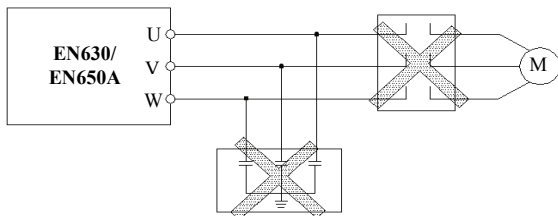
Fig.3-3 Forbid to use contactor and absorbing capacitor
