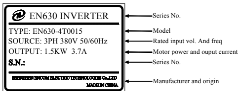
Fig.2-2 Nameplate
