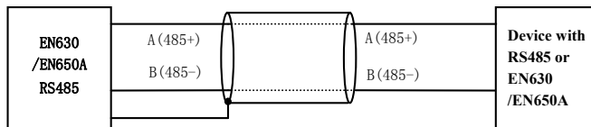
Fig.3-11 Communication terminal wiring
